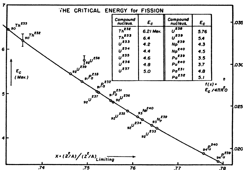
Fig. 24. The critical energy for fission, showing the values of the function f(x) = E_c / 4\pi r_0^2 and the assigned values of the critical energy E_c for the region of interest. The assignment was made to fit best the recent determinations of the thresholds for fission (see text).
