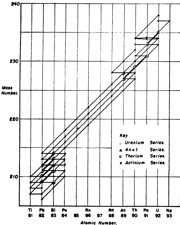
Fig. 21. The radioactive series.
