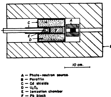
Fig. 19. Arrangement for observing the fast neutrons emitted by uranium. (Szilard and Zinn.)
