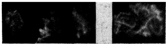
Fig. 50. Autoradiograph of slabs of silicon with small amounts of aluminum impurity. Each slab was irradiated with fast neutrons and placed on film. The exposed streaks are where the aluminum was changed to radioactive sodium which reveals its presence by the emission of beta rays. (See page 248.)
