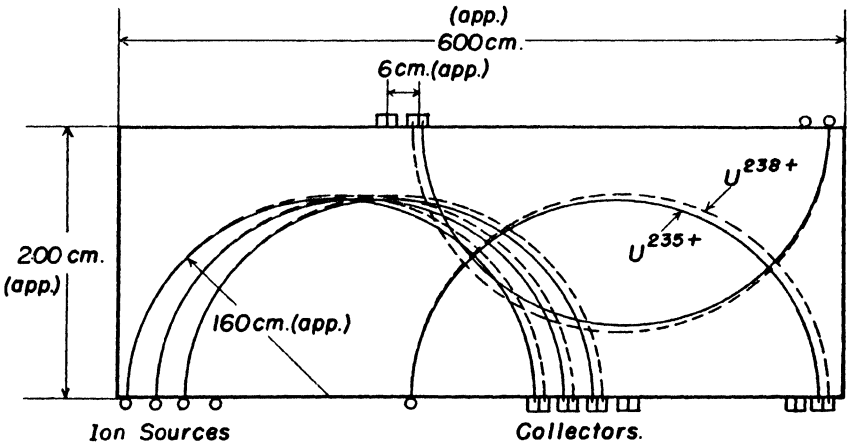
Fig. 38. Possible layout of a magnetic separator. Ion sources and collectors are placed along the long sides of a rectangular pole gap of a magnet in order to utilize the magnetic field to the best advantage and to have easy access to all parts. By proper dimensioning of the apparatus it should be possible to use about 100 ion sources per magnet.
