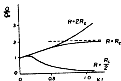
Fig. 32. The total number Q of neutrons in the sphere is shown as a function of kt for spheres of various radii. Q_0 is the number of neutrons initially concentrated at the origin. R_c is the critical radius (Adler).
