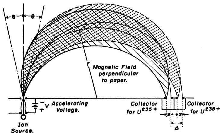
Fig. 35. Separation of isotopes by a Dempster type mass spectrometer. The ions ( U^{235+} and U^{238+} ) leave the ion source and after acceleration by a voltage V , enter a magnetic field H . The ions are approximately focussed after a deflection of 180^\circ by the magnetic field, the heavier ions further away from the entrance slit than the lighter ions, and are collected by separate collectors.
