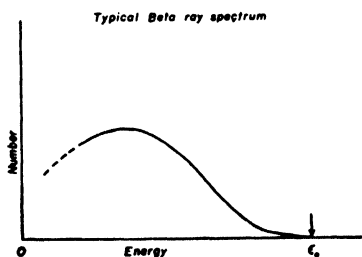
Fig. 11. Typical beta ray spectrum.
