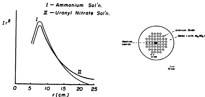
Fig. 17. The product of the intensity of neutrons and the square of the distance from the source is shown plotted as a function of the distance from the neutron source for a uranyl nitrate solution and an ammonium nitrate solution. (Von Halban, Joliot and Kowarski.)
