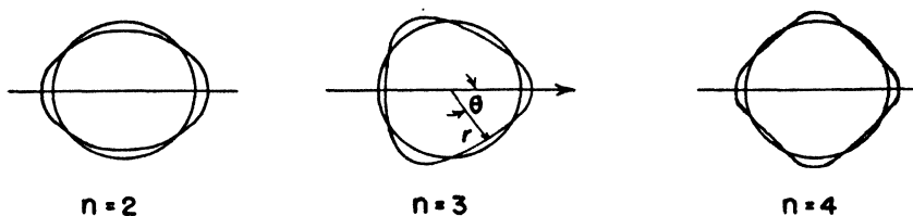
Fig. 25. Deformations of the nucleus corresponding to \alpha_2 , \alpha_3 , and \alpha_4 of Equation 15. The cases shown are for small values of the \alpha 's. For larger \alpha_2 the nucleus will develop a neck connecting two equal portions of the "liquid." For a given increase in surface area the deformation n=2 tends to decrease the electrostatic energy faster than any other deformation.
