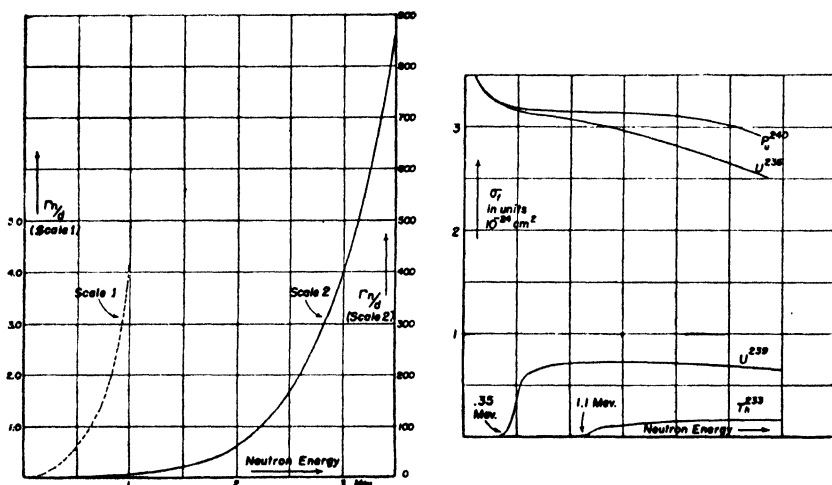
Fig. 30. The quantity \Gamma_n/d of equation 35 is plotted against the maximum energy of the emitted neutrons.
