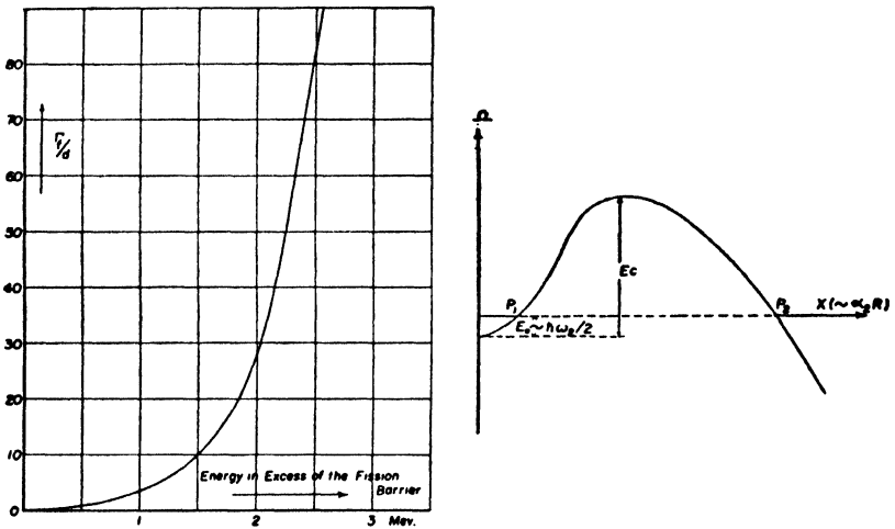
Fig. 28. (Bohr and Wheeler). The fission width divided by the level spacing of the compound nucleus is plotted against the energy in excess of the critical energy for fission. For example, with thermal neutrons on U^{235} , d is about 20 volts and the excess energy about 1.6 Mev so that \Gamma_f is about 200 volts, which is much larger than the radiation width.
