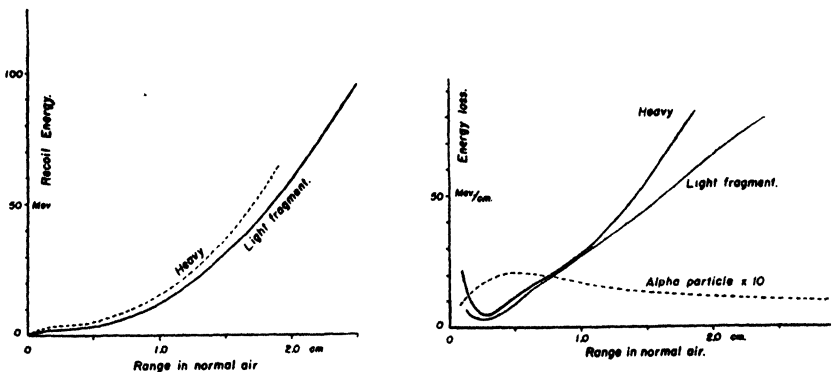
Fig. 7. Range energy curves for typical fission fragments. (Calculated from data of Bøggild, Brostrøm and T. Lauritsen.)
