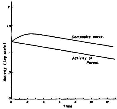
Fig. 14. Number vs. time for two radioactive substances with T_1 \sim 10T_2 .
