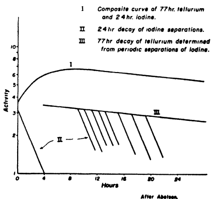
Fig. 16. Activity curves for radioactive decay of tellurium and iodine fractions. (Abelson.)
