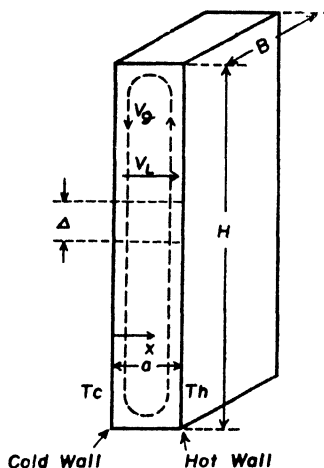
Fig. 45. Schematic diagram of a thermal diffusion column. The fluid containing the two isotopes to be separated is placed between two plane heat conducting walls which serve to establish a temperature gradient through the fluid. The direction of the convection flow ( v_g ) and the diffusion flow ( v_L ) is indicated. The end volumes at the top and bottom of the column are not shown.
