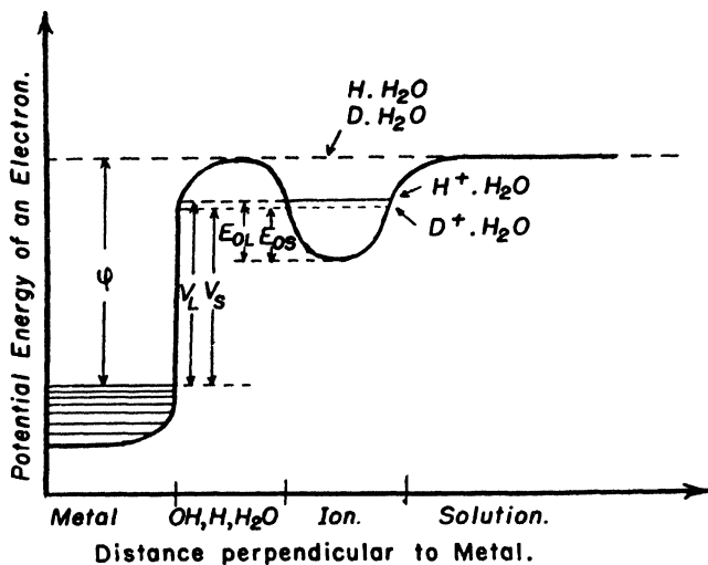
Fig. 41. Electron potential near a metal surface during electrolysis. A hydrated ion which approaches a cathode surface in order to be discharged is held at some distance from the surface by layers of H, OH and H 2 O molecules. The discharge can take place only by electrons leaving the metal and effectively overcoming the over voltage V (W. Walcher, Erg. d. exakt. Naturw. 18 , 155 (1939).)
