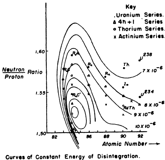
Fig. 22. Curves of constant disintegration energy (Heisenberg). The points for the 4n+1 series have been added.
