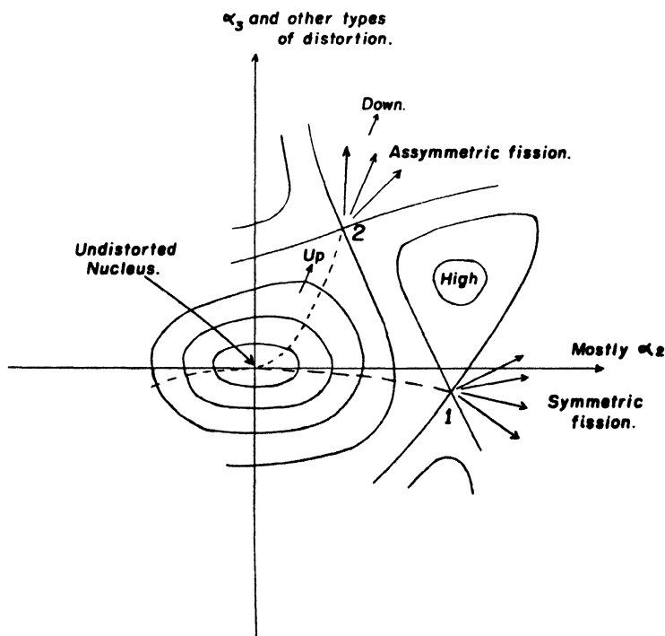
Fig. 26. Potential energy diagram for nuclear deformations. This shows the possibility of two different critical fission energies E_{o1} and E_{o2} , the first corresponding to a symmetric distortion and the second to division into unequal fragments. In the case shown here E_{o1} > E_{o2} which seems to be indicated by experiment.
