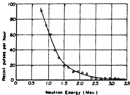
Fig. 20. The energy distribution of secondary neutrons accompanying uranium fission. (Zinn and Szilard.)
