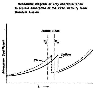
Fig. 10. Schematic diagram of X-ray characteristics to explain absorption of the 77-hour activity from uranium fission.
