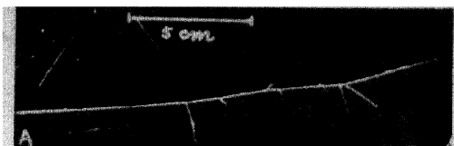
Fig. 5. Cloud chamber picture of a fission fragment recoiling in hydrogen. The large probability of nuclear collisions is clearly shown by the numerous branches. The range is amplified by the use of low pressure of hydrogen. The cloud chamber was filled with hydrogen gas plus vapor of one third alcohol and two thirds water, making a total pressure of 13 cm of mercury. (Bøggild, Brostrøm and T. Lauritsen, Det. Kgl. Danske Vid. Selskab, Math-fys. Medd. XVIII 4 (1940))
