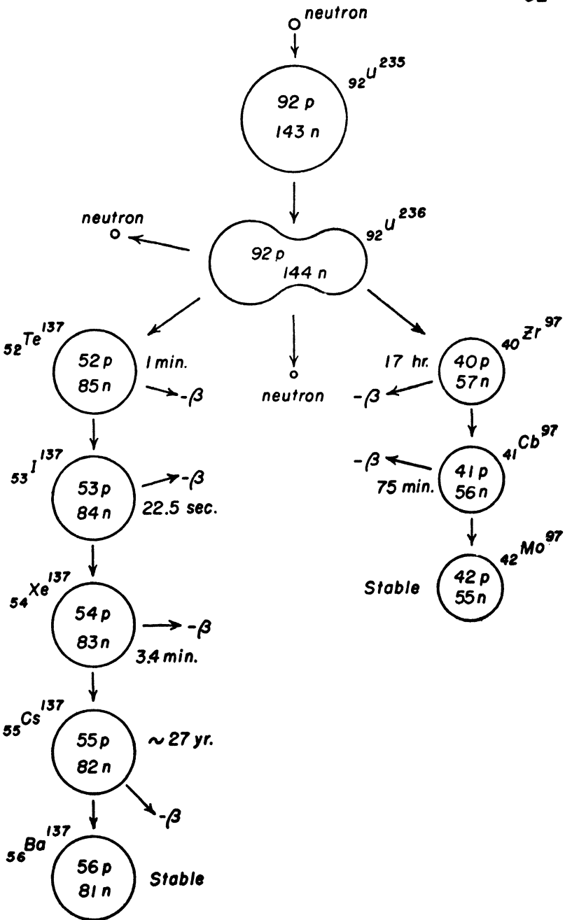
Fig. 9. Typical radioactive series from fission of \text{U}^{235} .
