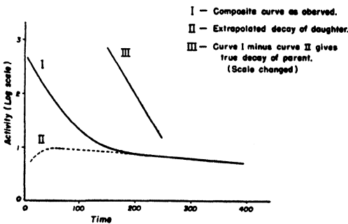
Fig. 13. Activity curve for fig. 12. Activity vs. time for decay of two radioactive substances with T_1 \sim 1/25 T_2 . (Meitner, Hahn and Strassmann.)
