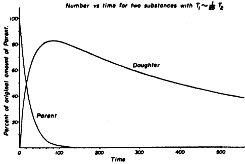
Fig. 12. Number vs. time for two radioactive substances with T_1 \sim 1/25 T_2 .
