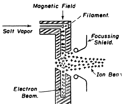
Fig. 36. Schematic cross-section of a possible arc type ion source. The salt vapor to be ionized flows down a capillary and is ionized by the beam of electrons which traverses the same capillary. At the opening of the capillary the mutual repulsion of the ion pushes them out of the arc so that by suitable focussing shields they can be drawn away from the source.
