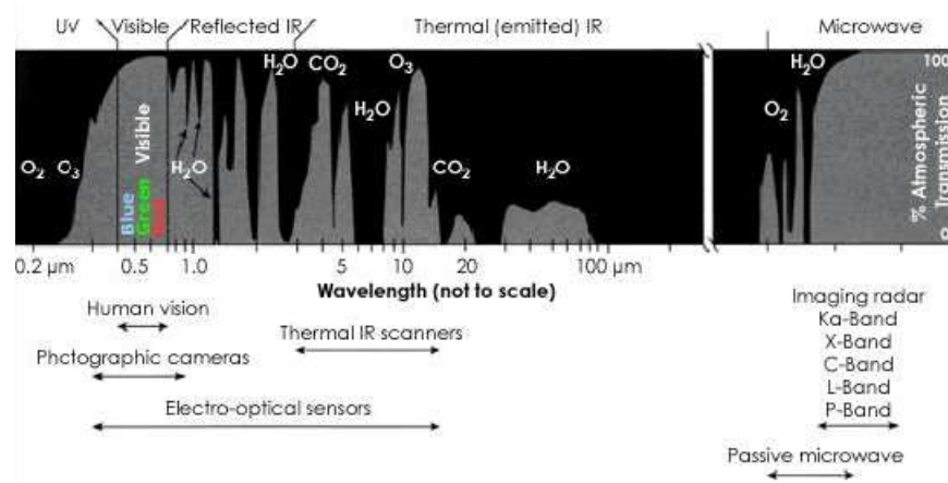
FIGURE 224 The transmittance of the atmosphere (NASA)
