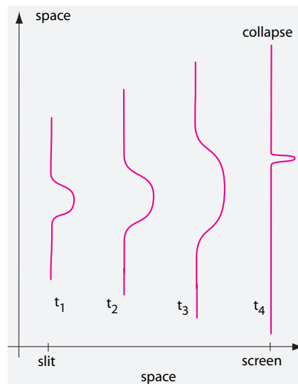
FIGURE 346 Quantum mechanical motion: an electron wave function (actually its module squared) from the moment it passes a slit until it hits a screen
