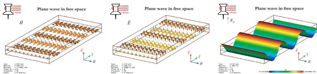
FIGURE 260 The general structure of a plane, monochromatic and linearly polarized electromagnetic wave at a specific instant of time
