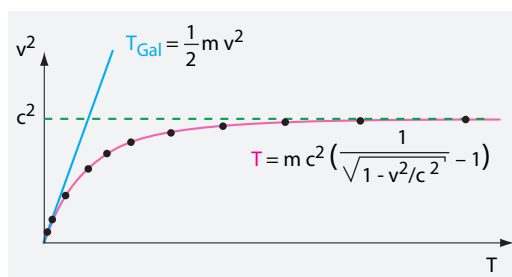
FIGURE 154 Experimental values (dots) for the electron velocity v as function of their kinetic energy T , compared with the prediction of Galilean physics (blue) and that of special relativity (red)
