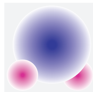
FIGURE 304 An artistic impression of a water molecule
