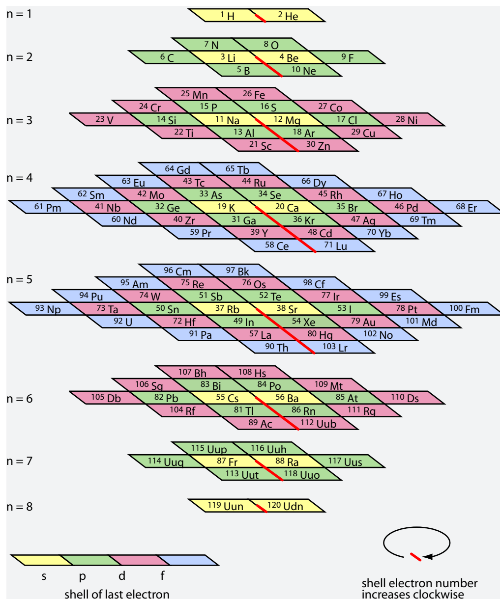
FIGURE 357 An unusual form of the periodic table of the elements
