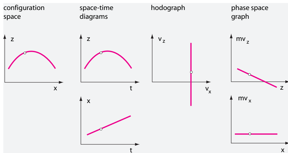
FIGURE 25 Various types of graphs describing the same path of a thrown stone
