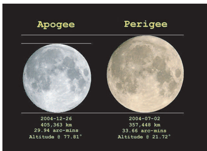
FIGURE 21 How the size of the Moon actually changes during its orbit (© Anthony Ayiomamitis)
