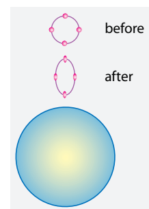
FIGURE 192 Tidal effects: the only effect bodies feel when falling
