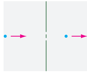
FIGURE 310 A particle and a screen with two nearby slits
