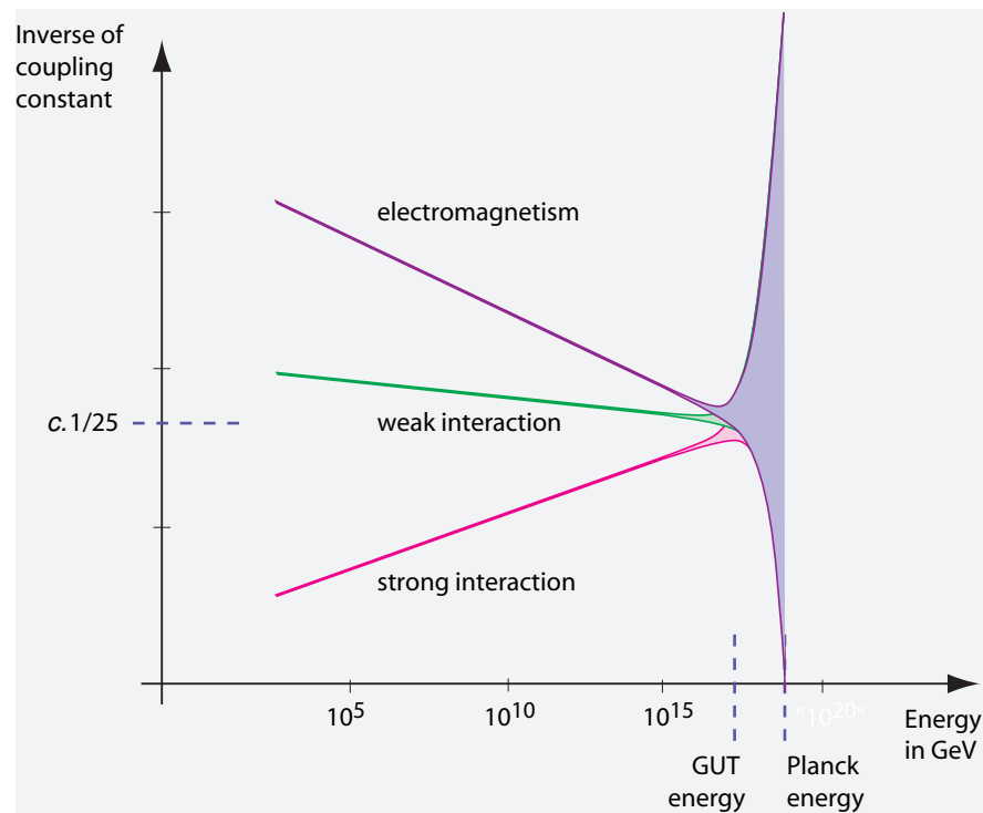
FIGURE 409 Coupling constants and their predicted spread as a function of energy
