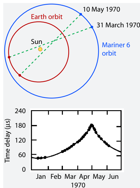
FIGURE 204 Time delay in radio signals – one of the experiments by Irwin Shapiro
