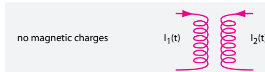
FIGURE 256 The second of Maxwell's equations
