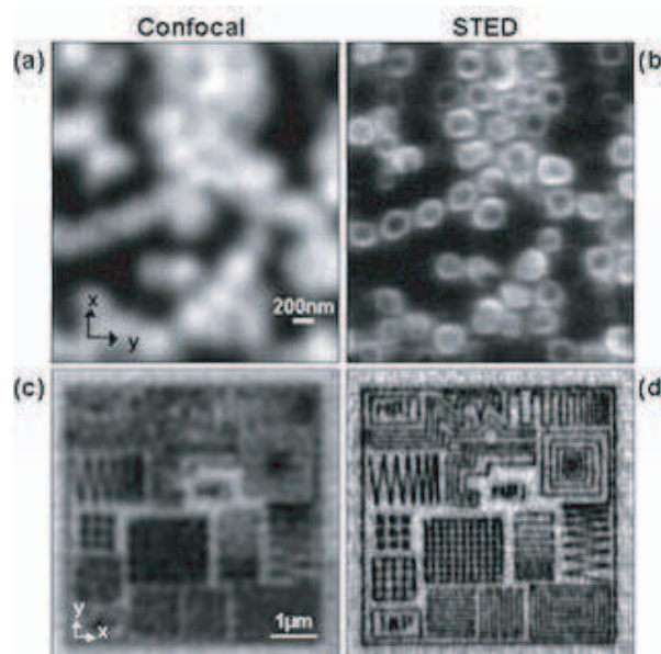
FIGURE 292 Sub-wavelength optical microscopy using stimulated emission depletion (© MPI für biophysikalische Chemie/Stefan Hell)
