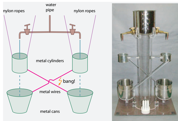
FIGURE 238 A simple Kelvin generator (photograph © Harald Chmela)
