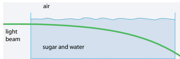
FIGURE 268 Sugar water bends light
