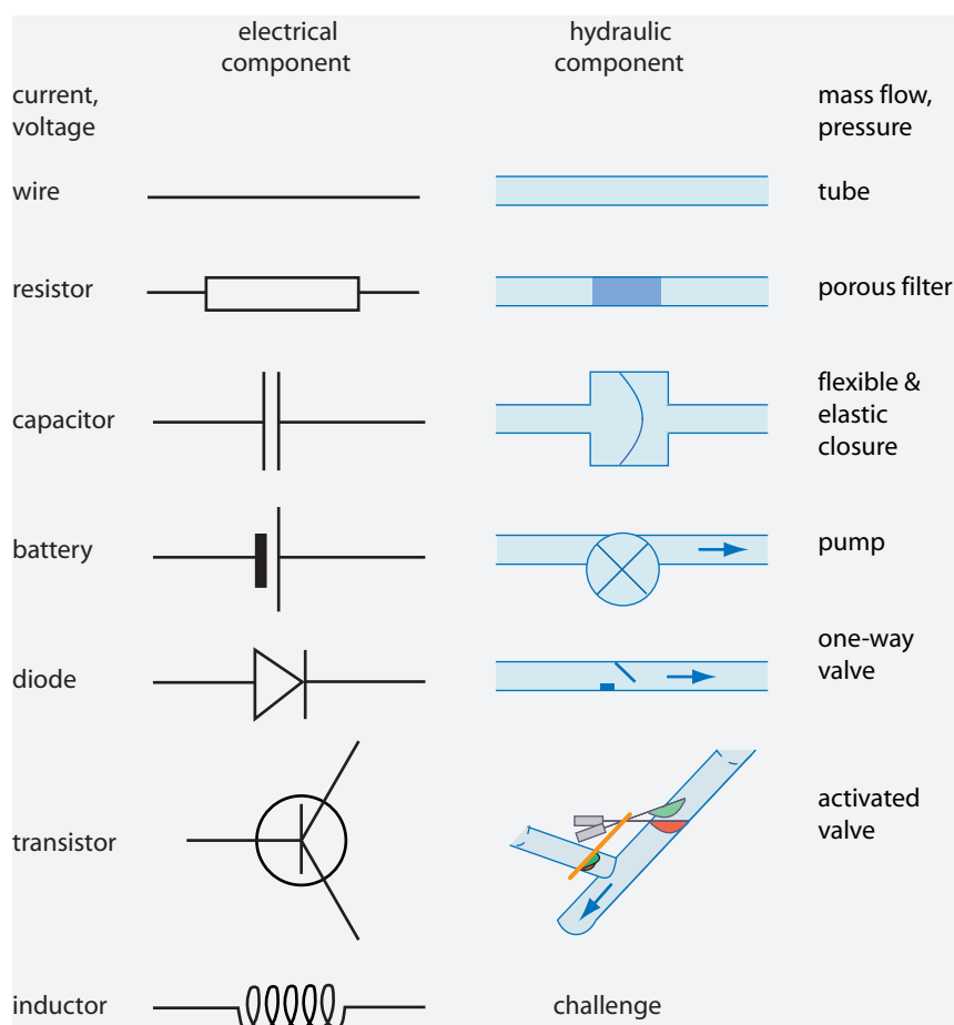
FIGURE 252 The correspondence of electronics and water flow
