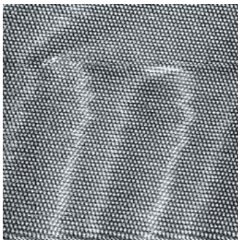
FIGURE 131 A 111 surface of a gold single crystal, every bright dot being an atom, with a surface dislocation (© CNRS)
