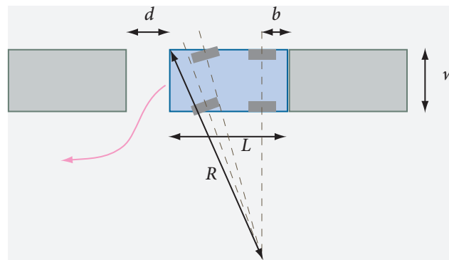
FIGURE 429 Leaving a parking space – the outer turning radius
