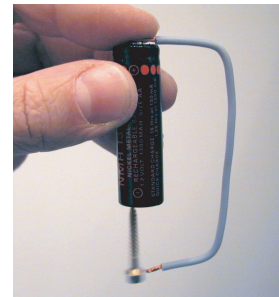
FIGURE 251 The simplest motor (© Stefan Kluge)
