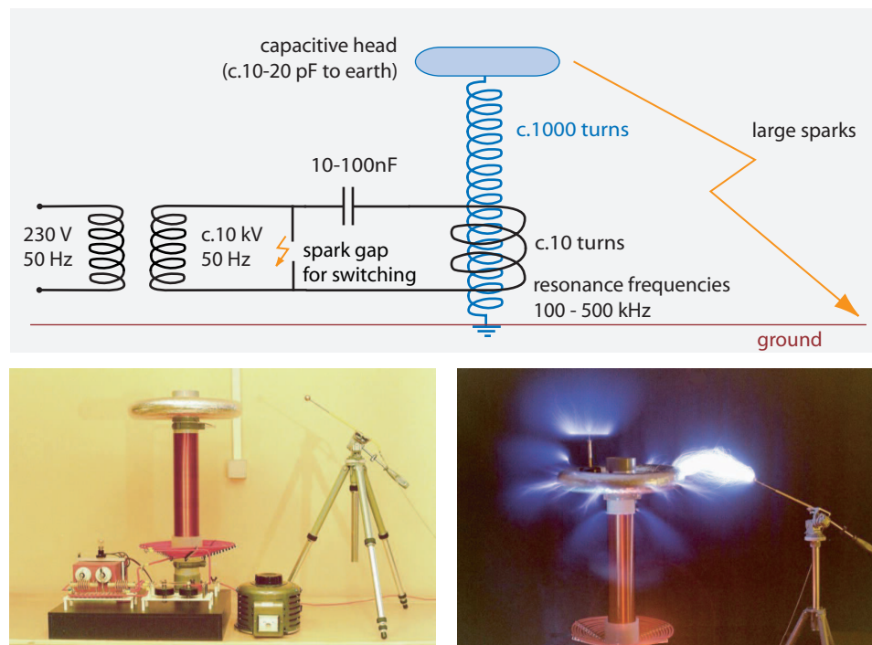
FIGURE 247 The schematics, the realization and the operation of a Tesla coil, including spark and corona discharges (photographs © Robert Billon)
