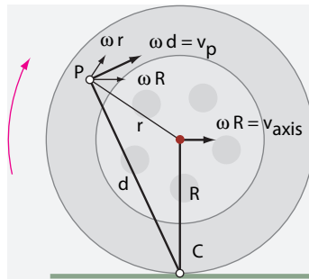
FIGURE 39 The velocities and unit vectors for a rolling wheel
