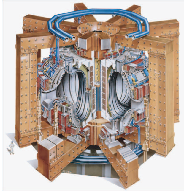
FIGURE 380 A simplified drawing of the Joint European Torus in operation at Culham, showing the large toroidal chamber and the magnets for the plasma confinement (© EFDA-JET)
