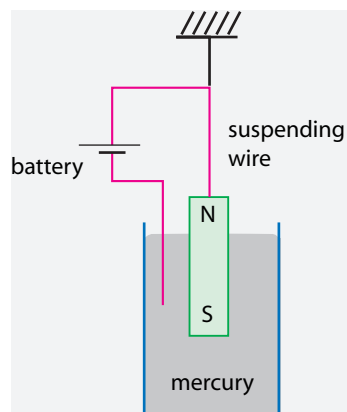
FIGURE 250 A unipolar motor
