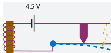
FIGURE 440 How to get shocks from 4.5 V
