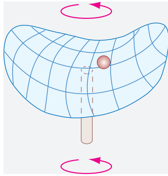
FIGURE 298 Trapping a metal sphere using a variable speed drill and a plastic saddle
