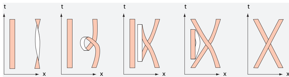
FIGURE 344 Belts in space-time: rotation and antiparticles
