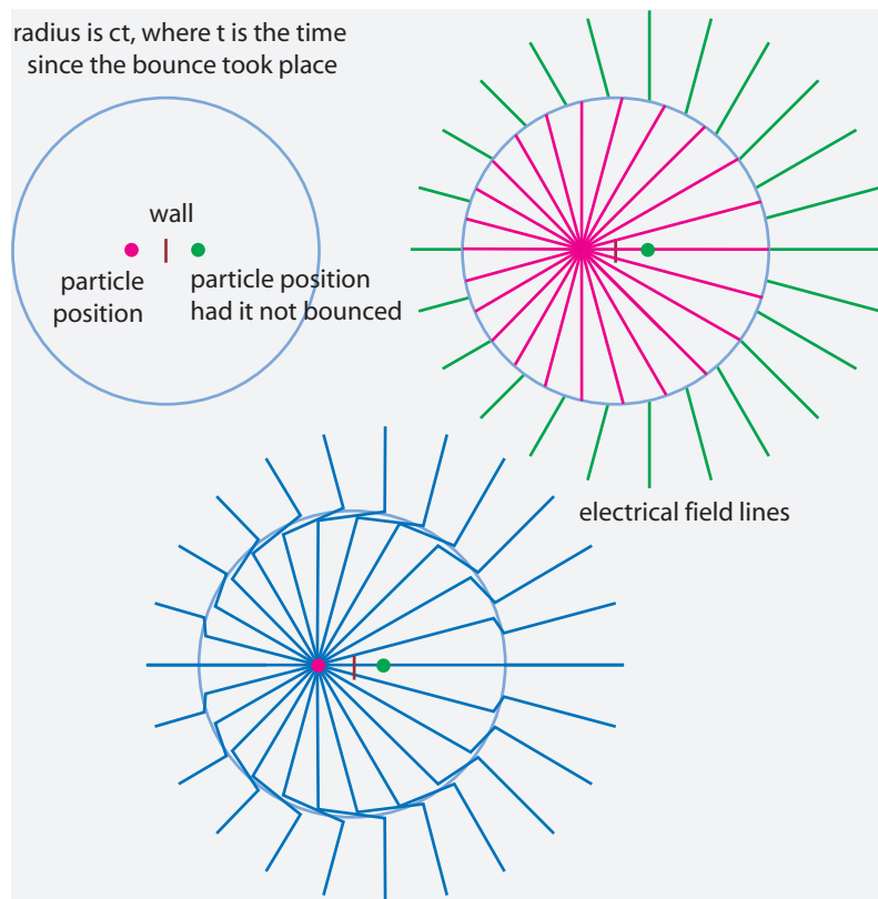
FIGURE 266 Constructing, in three steps, the electrical field around a particle bouncing from a wall
