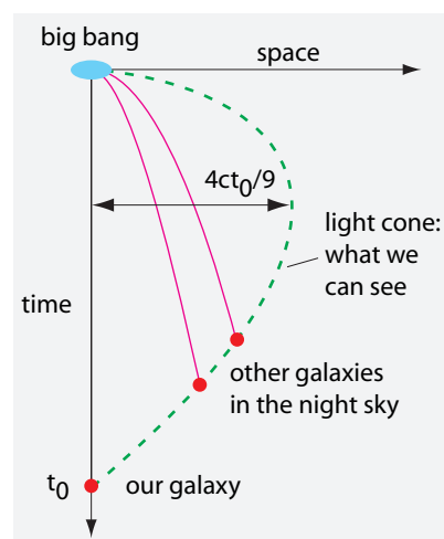
FIGURE 412 The speed and distance of remote galaxies
