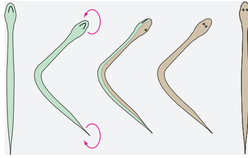
FIGURE 37 How a snake turns itself around its axis
