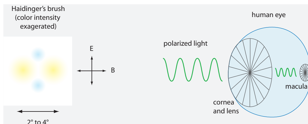
FIGURE 265 Haidinger's brush and its origin in the human eye
