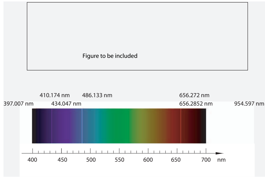
FIGURE 331 The non-relativistic energy levels and the visible spectrum of hydrogen (NASA)
