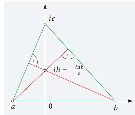
FIGURE 419 A property of triangles easily provable with complex numbers
