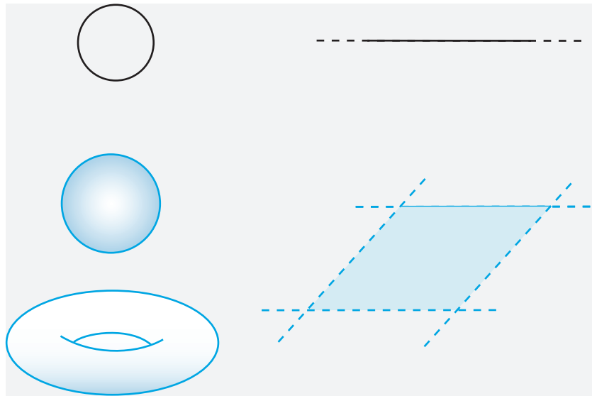
FIGURE 423 Compact (left) and noncompact (right) manifolds of various dimensions
