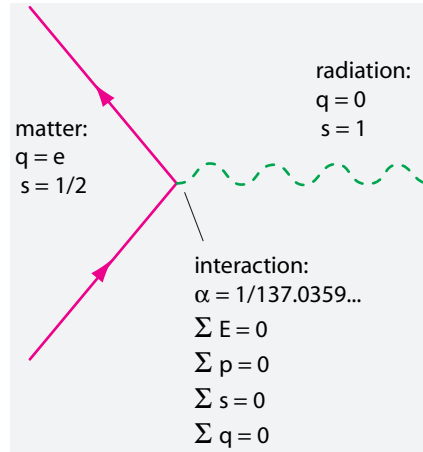
FIGURE 366 QED as perturbation theory in space-time
