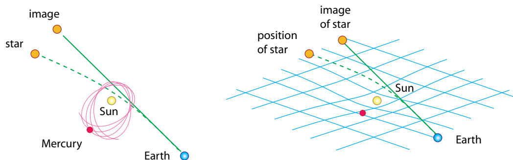
FIGURE 193 The mattress model of space: the path of a light beam and of a satellite near a spherical mass
