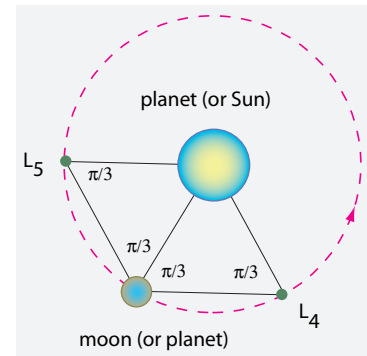
FIGURE 76 The two stable Lagrangian points
