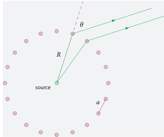
FIGURE 327 On the quantization of angular momentum
