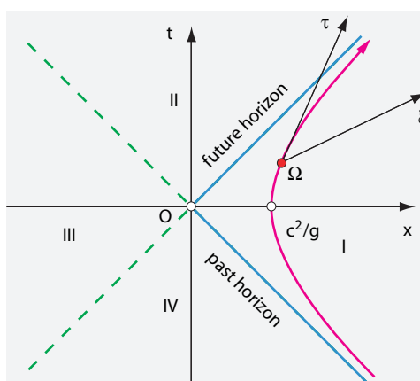
FIGURE 186 Hyperbolic motion and event horizons
