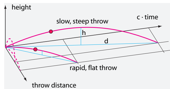
FIGURE 194 All paths of flying stones have the same curvature in space-time
