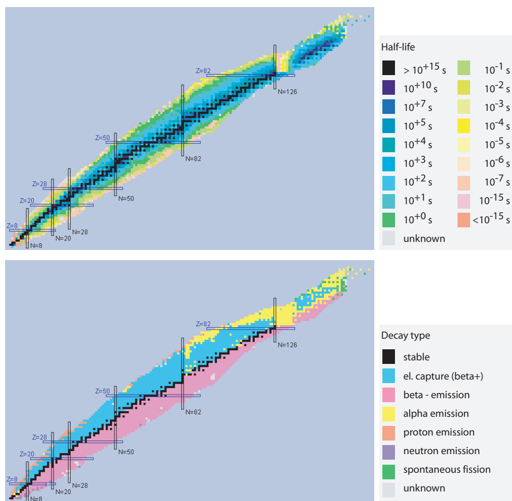
FIGURE 372 All known nuclides with their lifetimes (above) and main decay modes (BELOW, data from http://www.nndc.bnl.gov/nudat2 )
