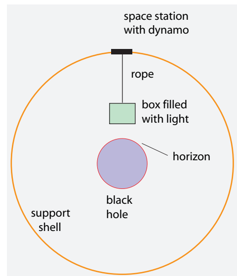
FIGURE 368 A Gedanken experiment allowing to deduce the existence of black hole radiation
