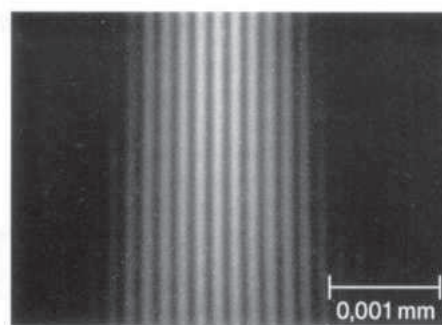
FIGURE 325 Electrons beams diffract and interfere at multiple slits (© Claus Jönsson)
