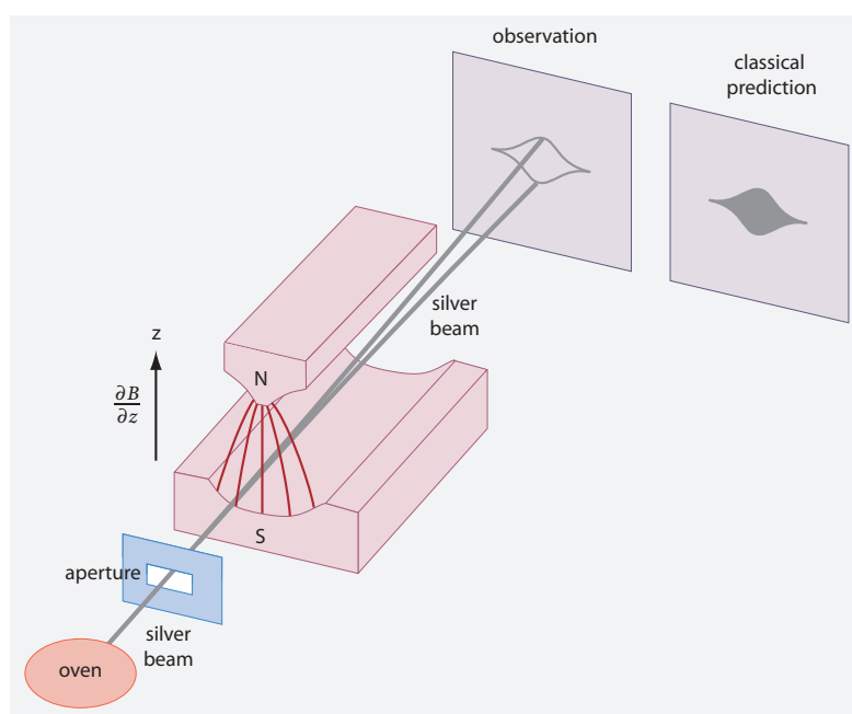
FIGURE 328 The Stern-Gerlach experiment
