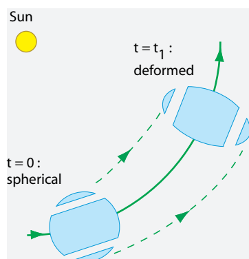
FIGURE 78 Tidal deformations due to gravity
