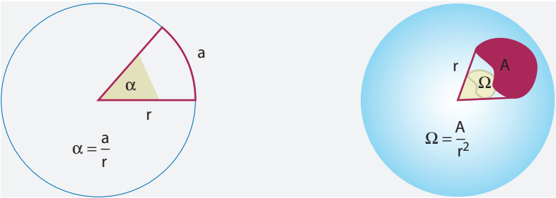
FIGURE 19 The definition of plane and solid angles
