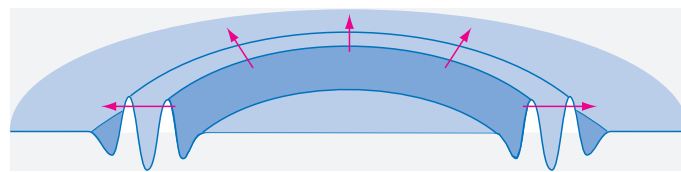
FIGURE 110 An impossible water wave: the centre is never flat
