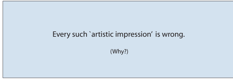
FIGURE 345 An artist's impressions of a macroscopic superposition is impossible
