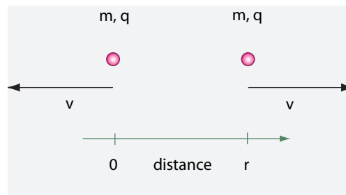
FIGURE 257 Charged particles after a collision
