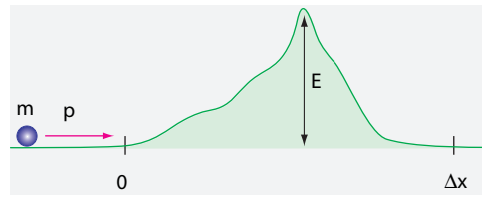
FIGURE 305 Hills are never high enough
