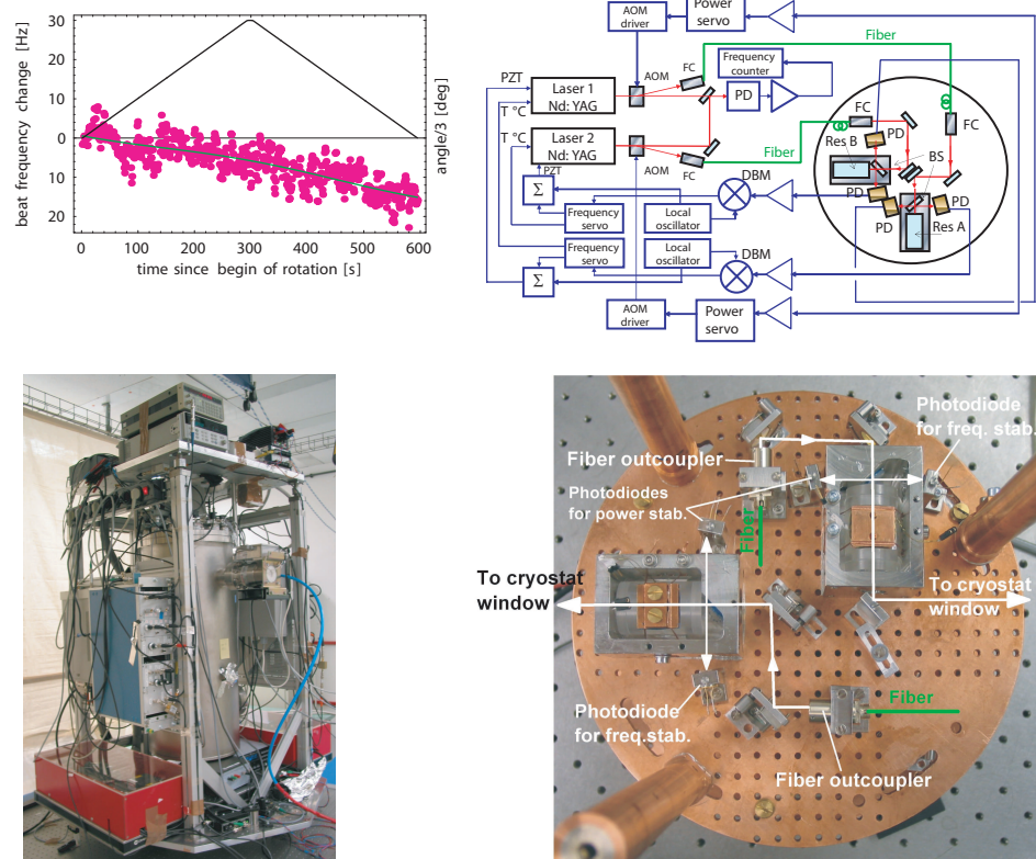
FIGURE 156 The result, the schematics and the cryostat set-up for the most precise Michelson–Morley experiment performed to date (© Stephan Schiller)
