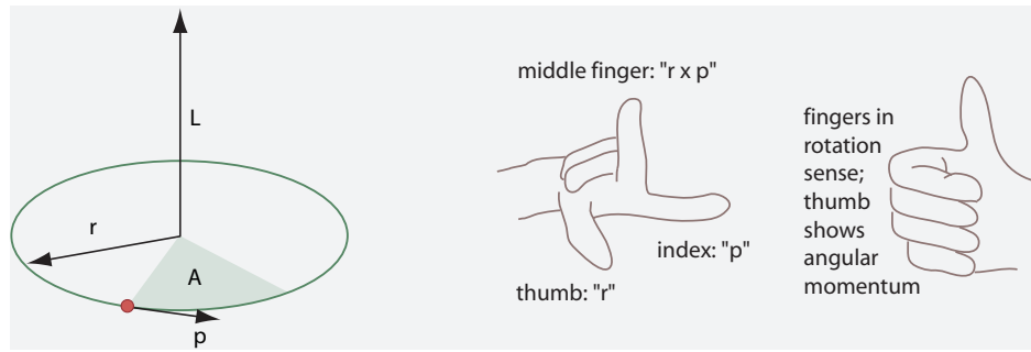
FIGURE 36 Angular momentum and the two versions of the right-hand rule
