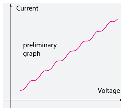
FIGURE 324 Steps in the flow of electricity in metals
