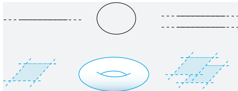
FIGURE 424 Simply connected (left), multiply connected (centre) and disconnected (right) manifolds of one (above) and two (below) dimensions
