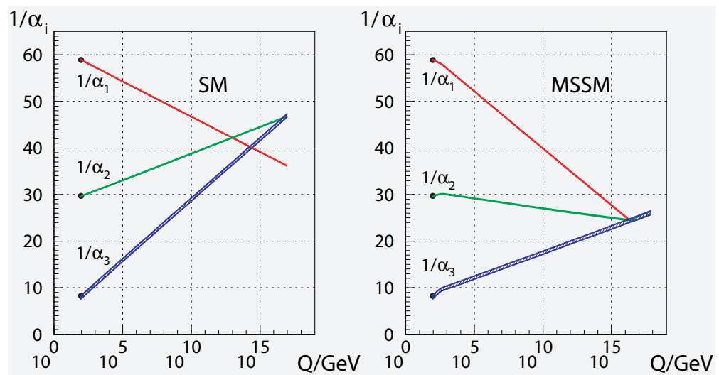
FIGURE 384 The behaviour of the three coupling constants with energy for the standard model (left) and for the minimal supersymmetric model (right) (© Wim de Boer)
