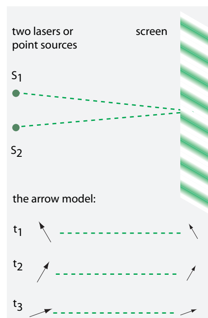
FIGURE 318 Interference and the description of light with arrows (at one particular instant of time)
