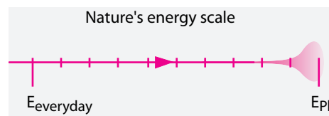
FIGURE 416 Planck effects make the energy axis an approximation
