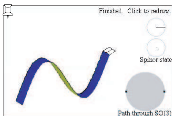
FIGURE 337 The belt trick (© Greg Egan)
