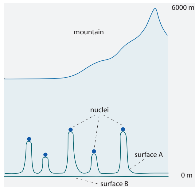
FIGURE 189 The mountain attempt to exceed the maximum mass flow value
