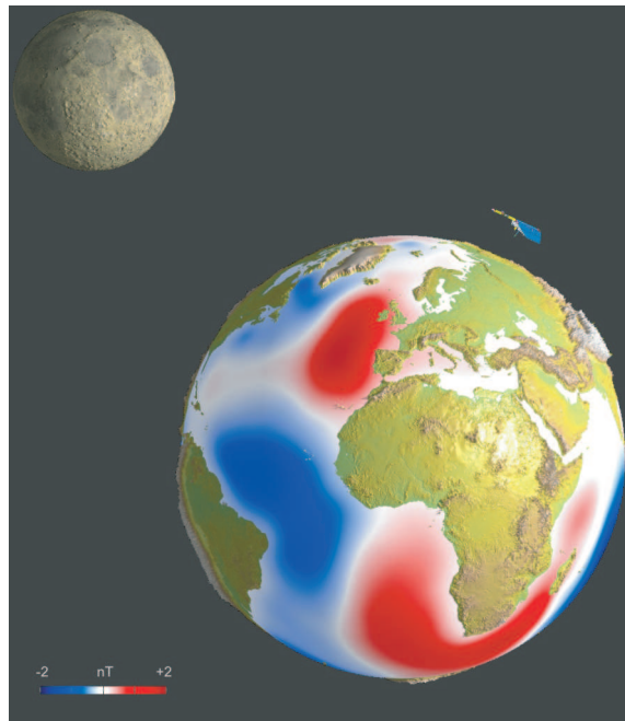
FIGURE 249 The magnetic field due to the tides (© Stefan Maus)
