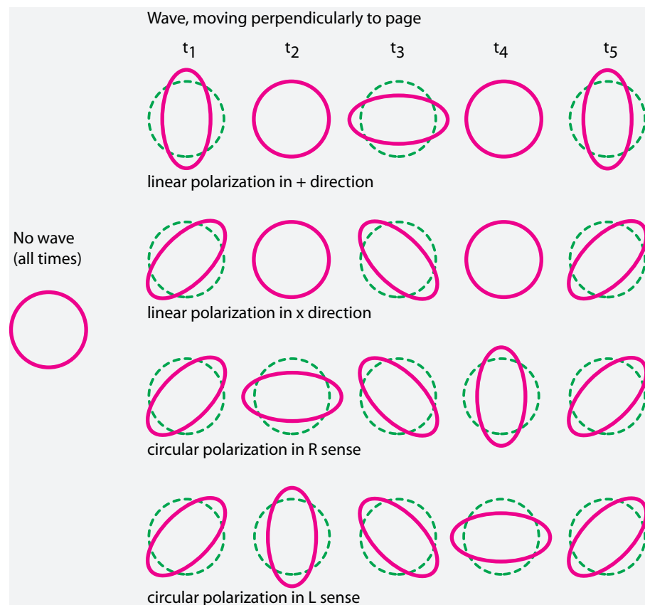
FIGURE 200 Effects on a circular or spherical body due to a plane gravitational wave moving in a direction perpendicular to the page
