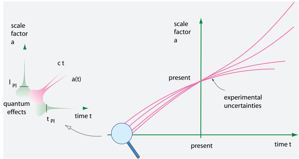
FIGURE 221 The evolution of the universe's scale a for different values of its mass density
