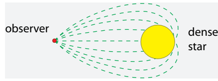
FIGURE 232 Motion of some light rays from a dense body to an observer
