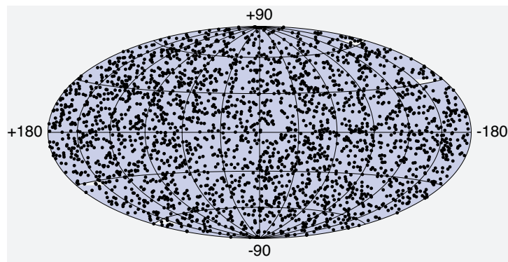
FIGURE 369 The location of the 2704 gamma ray bursts observed in the sky between 1991 and 2000 by the BATSE satellite; the galactic plane is horizontal (NASA)
