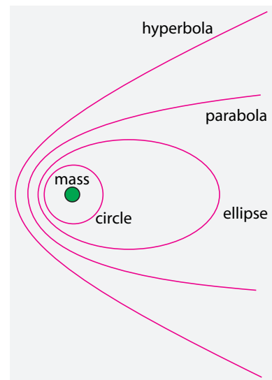
FIGURE 75 The possible orbits due to universal gravity
