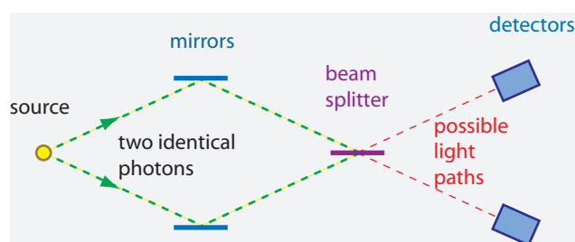
FIGURE 334 Two photons and interference
