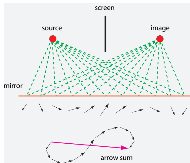
FIGURE 319 Light reflected by a mirror and the corresponding arrows (at one particular instant of time)
