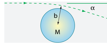
FIGURE 273 Masses bend light
