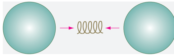
FIGURE 199 A Gedanken experiment showing the necessity of gravity waves
