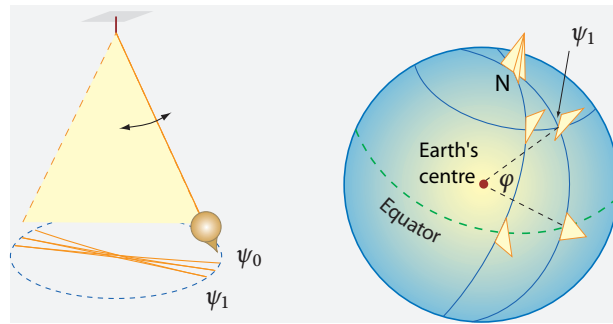
FIGURE 45 The turning motion of a pendulum showing the rotation of the Earth
