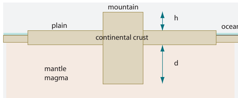
FIGURE 54 A simple model for continents and mountains
