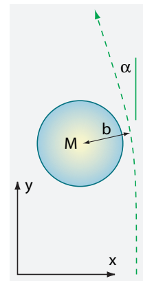
FIGURE 203 Calculating the bending of light by a mass
