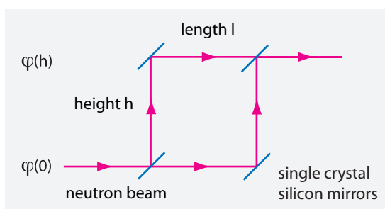
FIGURE 367 The weakness of gravitation
