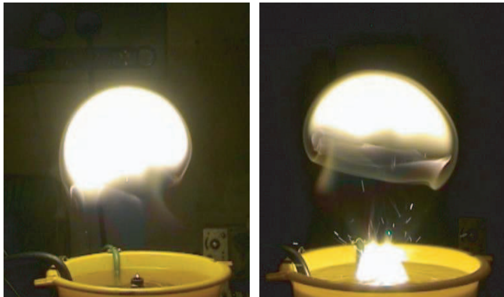
FIGURE 296 A floating plasma cloud produced in the laboratory (© Sergei Emelin and Alexei Pirozerski)
