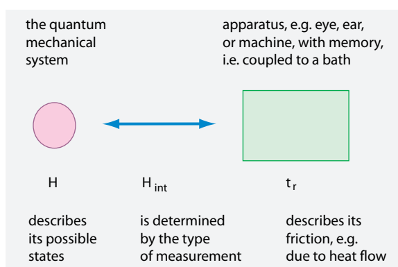
FIGURE 349 The concepts used in the description of measurements
