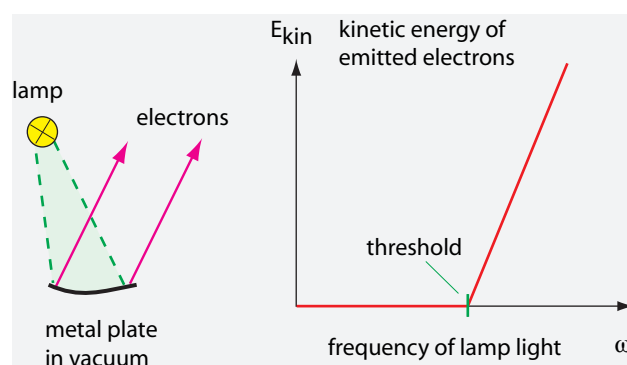
FIGURE 316 The kinetic energy of electrons emitted in the photoelectric effect
