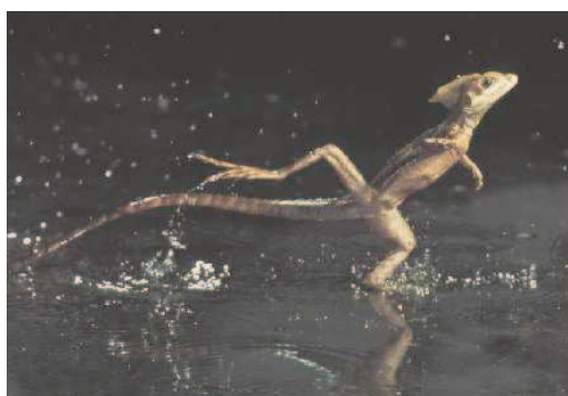
FIGURE 64 A basilisk lizard ( Basiliscus basiliscus ) running on water, showing how the propulsing leg pushes into the water (© TERRA)
