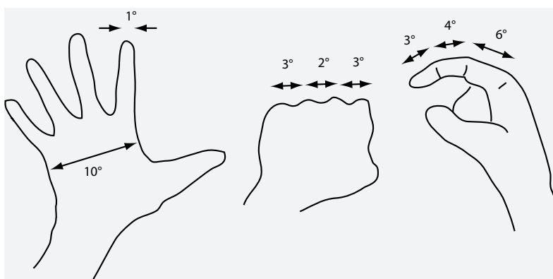
FIGURE 432 The angles defined by the hands against the sky, when the arms are extended
