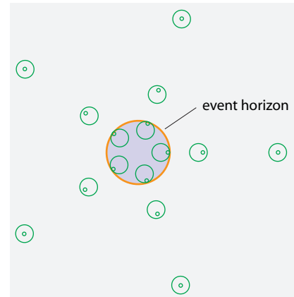
FIGURE 228 The light cones in the equatorial plane around a non-rotating black hole, seen from above
