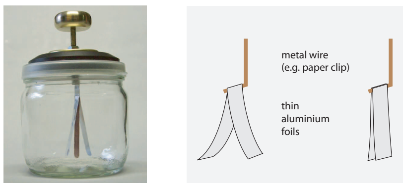
FIGURE 373 An electrostatic demonstrator (© Harald Chmela) and its charged (left) and uncharged state (right)
