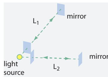
FIGURE 202 Detection of gravitational waves
