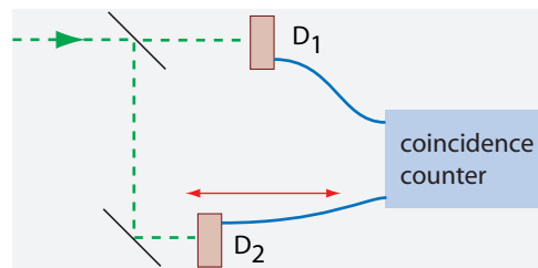
FIGURE 315 How to measure photon statistics: with an electronic coincidence counter and the variation by varying the geometrical position of a detector
