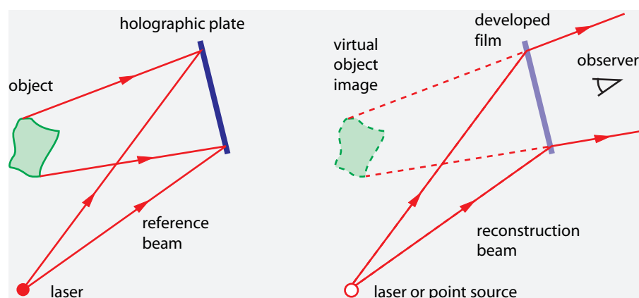
FIGURE 291 The recording and the observation of a hologram
