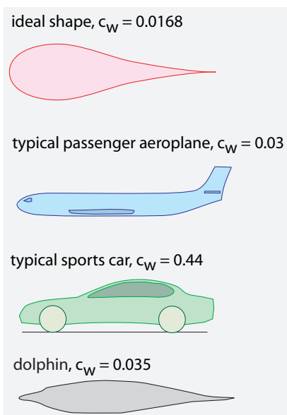
FIGURE 90 Shapes and air/water resistance
