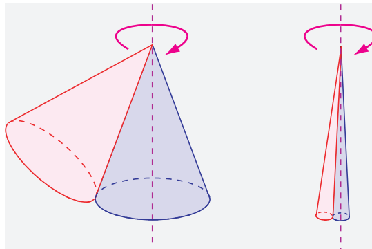
FIGURE 336 An argument showing why rotations by 4\pi are equivalent to no rotation at all
