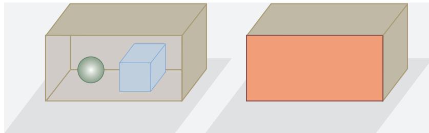
FIGURE 293 Bodies inside an oven at room temperature (left) and red hot (right)
