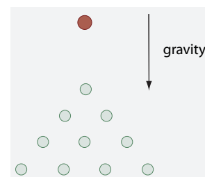
FIGURE 348 A system showing probabilistic behaviour
