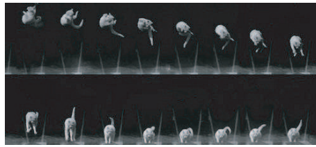
FIGURE 392 Cats can turn themselves, even with no initial angular momentum (photographs by Etienne-Jules Marey, 1894)
