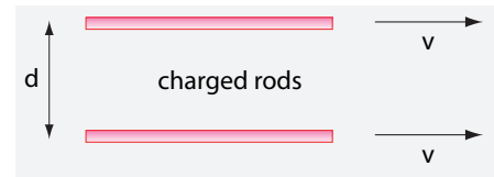
FIGURE 246 The relativistic aspect of magnetism
