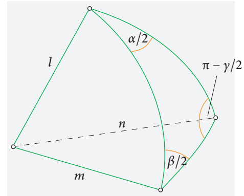
FIGURE 420 Combinations of rotations
