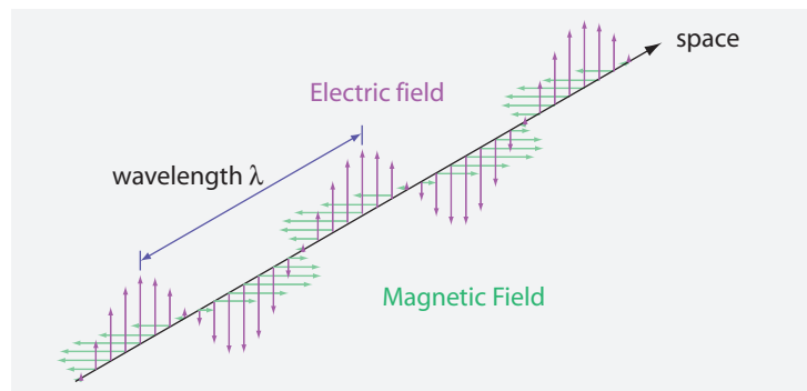
FIGURE 260 The general structure of a plane, monochromatic and linearly polarized electromagnetic wave at a specific instant of time
