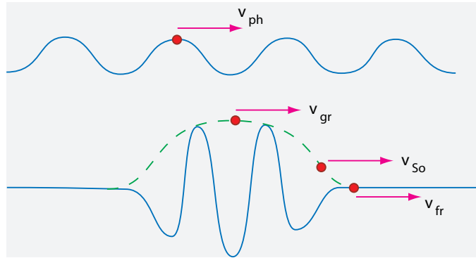
FIGURE 283 The definition of important velocities in wave phenomena
