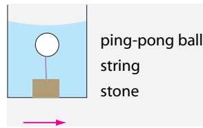
FIGURE 60 How does the ball move when the jar is accelerated?
