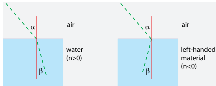
FIGURE 284 Positive and negative indices of refraction
