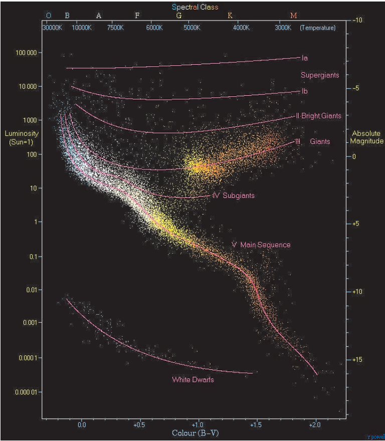
FIGURE 219 The Hertzsprung–Russell diagram (© Richard Powell)
