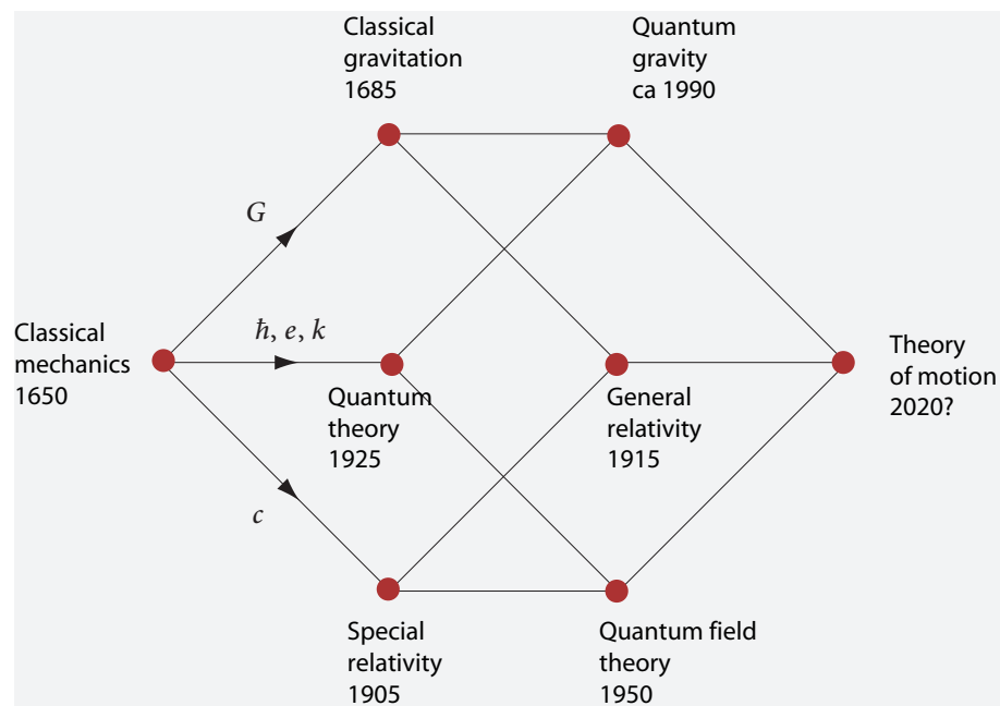
FIGURE 385 A simplified history of the description of motion in physics, by giving the limits to motion included in each description
