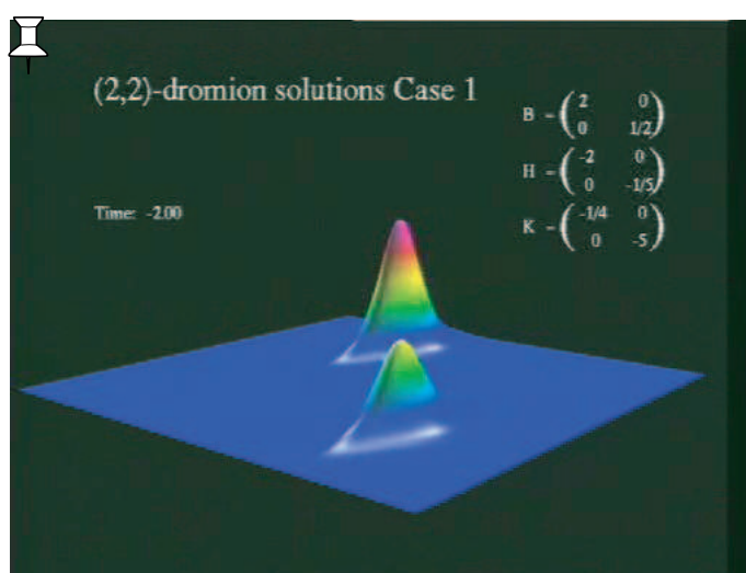
FIGURE 115 The calculated motion of a dromion across a two-dimensional substrate (© Jarmo Hietarinta)
