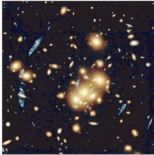
FIGURE 227 Multiple blue images of a galaxy formed by the yellow cluster CL0024+1654 (NASA)
