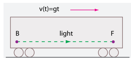
FIGURE 190 Inside an accelerating train or bus
