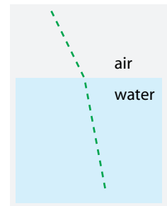
FIGURE 321 If light were made of little stones, they would move faster inside water
