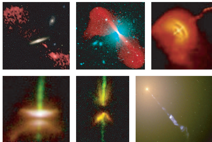
FIGURE 215 Rotating clouds emitting jets along their axis; top row: a composite image (visible and infrared) of the galaxy 0313-192, the galaxy 3C296, and the Vela pulsar; bottom row: the star in formation HH30, the star in formation DG Tauri B, and a black hole jet from the galaxy M87 (all NASA)
