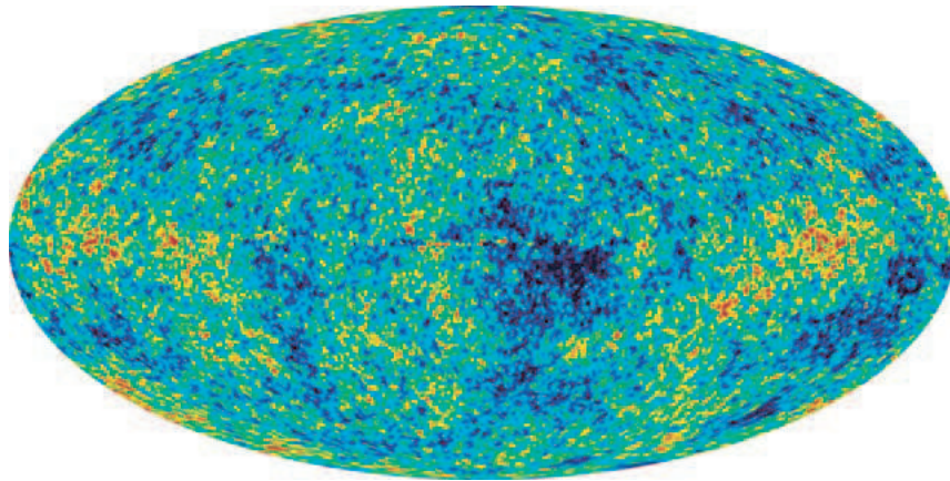
FIGURE 223 The fluctuations of the cosmic background radiation (WMAP/NASA)
