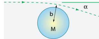
FIGURE 82 Masses bend light
