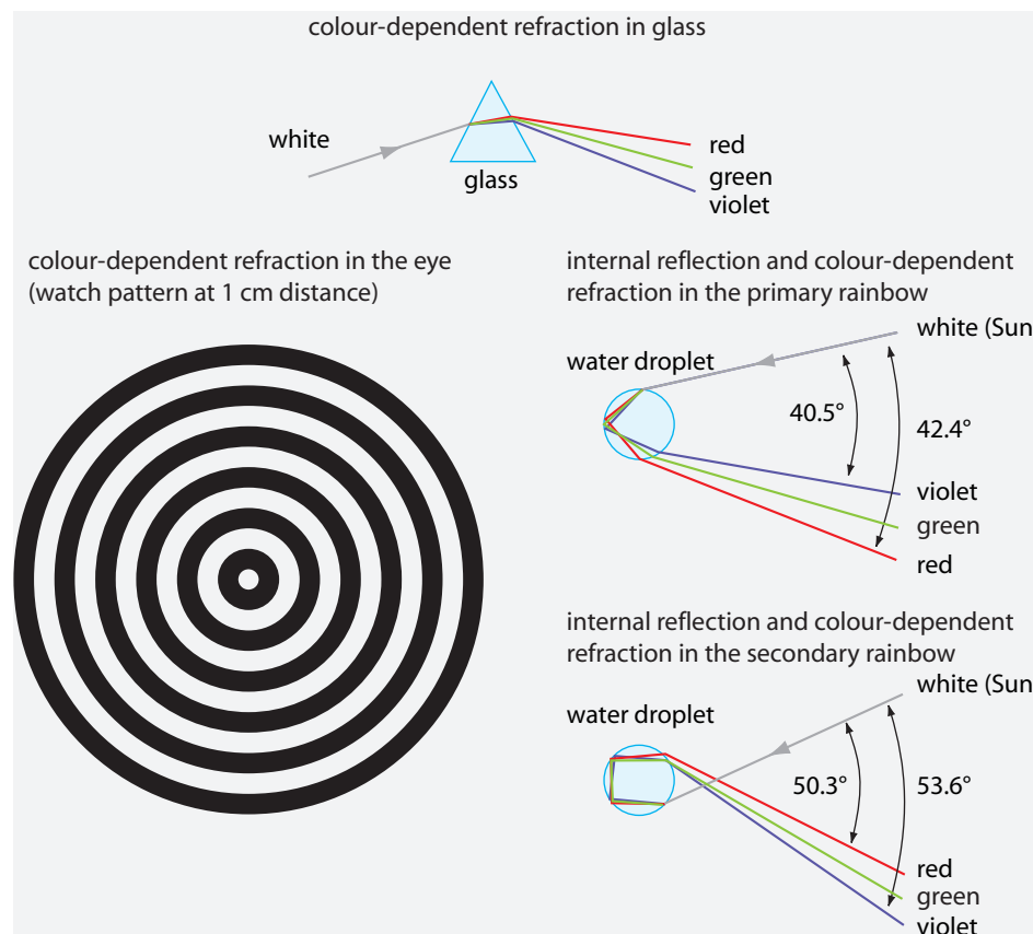
FIGURE 280 Proving that white light is a mixture of colours (angles much exaggerated!)
