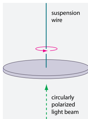
FIGURE 278 Light can rotate objects
