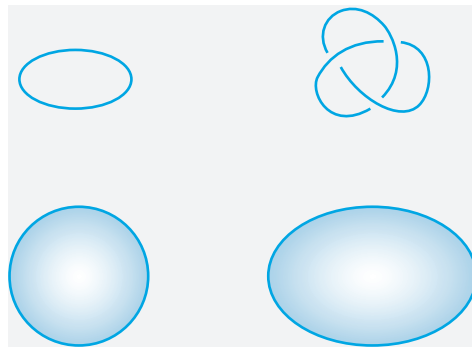
FIGURE 425 Examples of homeomorphic pairs of manifolds
