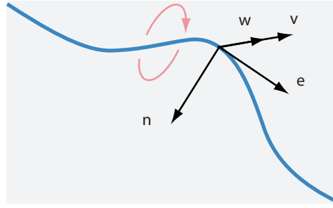
FIGURE 400 The mutually perpendicular tangent \mathbf{e} , normal \mathbf{n} , torsion \mathbf{w} and velocity \mathbf{v} of a vortex in a rotating fluid
