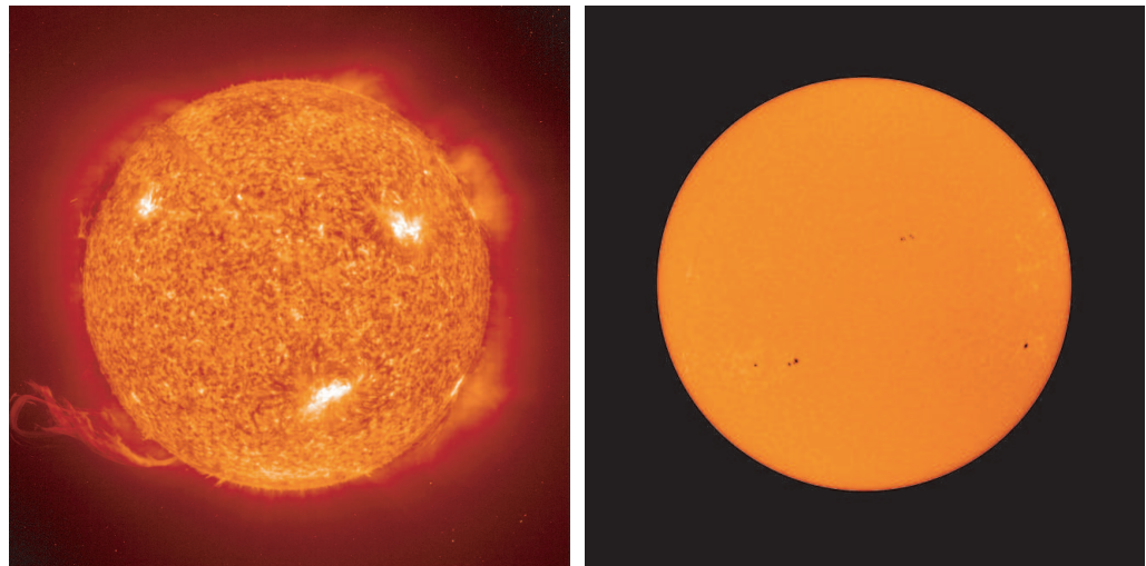
FIGURE 379 Photographs of the Sun at wavelengths of 30.4 nm (in the extreme ultraviolet, left) and around 677 nm (visible light, right, at a different date), by the SOHO mission (ESA and NASA)
