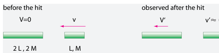
FIGURE 56 An elastic collision that seems not to obey energy conservation
