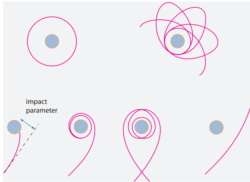
FIGURE 229 Motions of uncharged objects around a non-rotating black hole – for different impact parameters and initial velocities
