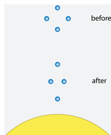
FIGURE 79 The origin of tides
