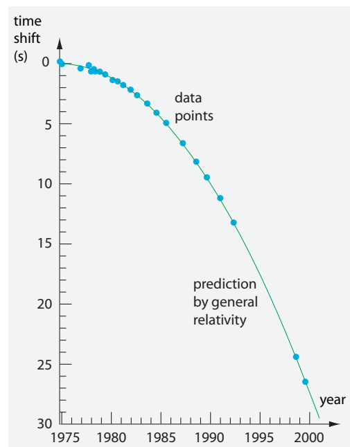
FIGURE 201 Comparison between measured time delay for the periastron of the binary pulsar PSR 1913+16 and the prediction due to energy loss by gravitational radiation
