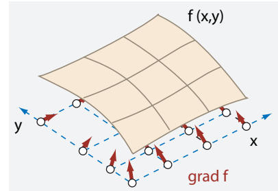
FIGURE 69 The potential and the gradient
