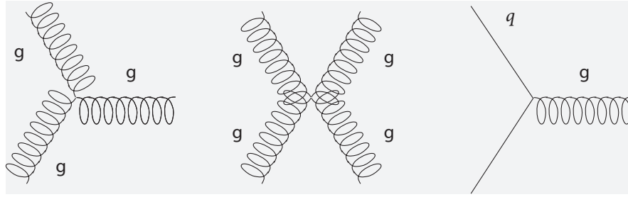
FIGURE 383 The essence of the QCD Lagrangian
