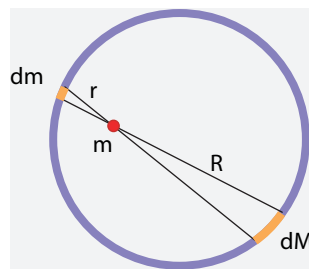
FIGURE 88 The vanishing of gravitational force inside a spherical shell of matter
