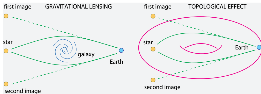
FIGURE 225 How one star can lead to several images
