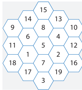
FIGURE 302 The only magic hexagon
