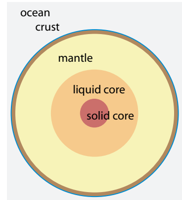
FIGURE 297 The structure of our planet
