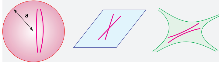
FIGURE 209 Curvature (in two dimensions) and geodesic behaviour
