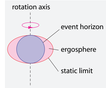
FIGURE 231 The ergosphere of a rotating black hole
