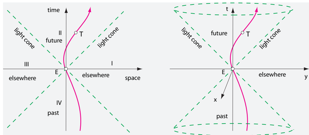
FIGURE 159 A space-time diagram for a moving object T seen from an inertial observer O in the case of one and two spatial dimensions
