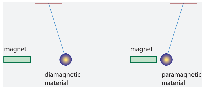
FIGURE 245 The two basic types of magnetic material behaviour (tested in an inhomogeneous field): diamagnetism and paramagnetism
