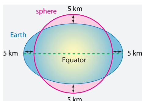
FIGURE 43 Earth's deviation from spherical shape due to its rotation
