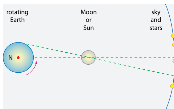
FIGURE 42 The parallax – not drawn to scale
