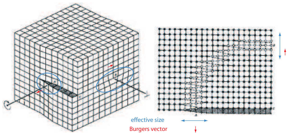
FIGURE 402 The two pure dislocation types: edge and screw dislocations
